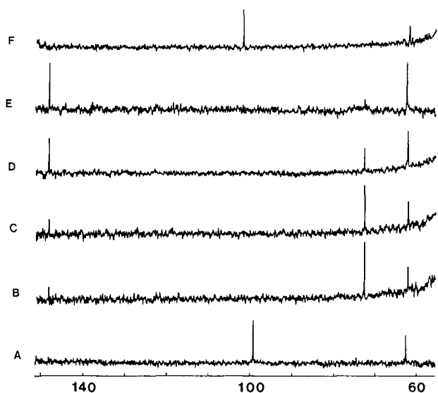
Figure 1. ^{13}\text{C} NMR spectra for the 4a\text{-}^{13}\text{C} intermediates described above, at -30\text{ }^\circ\text{C} . Chemical shifts are referenced to internal \text{CD}_3\text{OH} (49.0 ppm). The signal at 61.5 ppm is due to Tris buffer (20 mM): (A) [4a\text{-}^{13}\text{C}] -6-methyltetrahydropterin ( 1 ) prior to addition of PAH and phenylalanine; (B) spectrum acquired after mixing with \text{PAH}^4 t = 19\text{--}54 min (100 scans); (C) t = 64\text{--}170 min (260 scans); (D) t = 228\text{--}258 min (200 scans); (E) t = 360\text{--}400 min (100 scans); (F) solution after 580 min, allowed to warm to 30\text{ }^\circ\text{C} for 3 h (100 scans).
